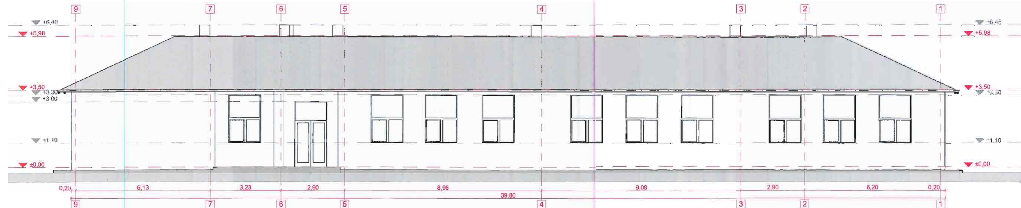
FATADA PRINCIPALA
